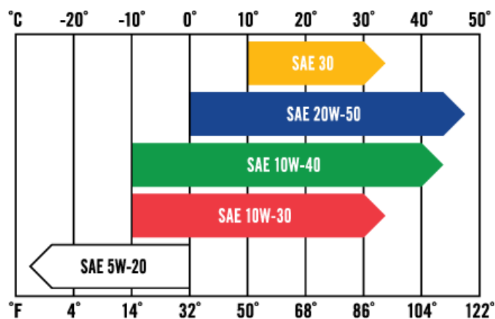
Chart of SAE oil classes according to external temperatures
